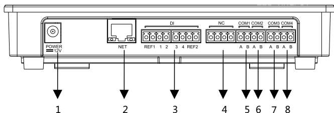
Figure 4.1-1 Schematic Diagram of Ports on the Bottom Surface of Ezlogger Pro
