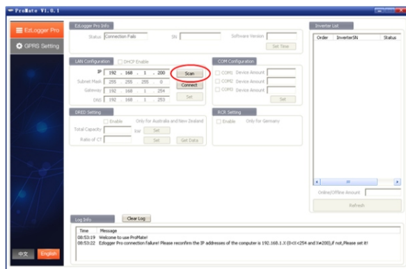
Figure 5.2-1 Connecting ProMate to EzLogger Pro by Scanning
