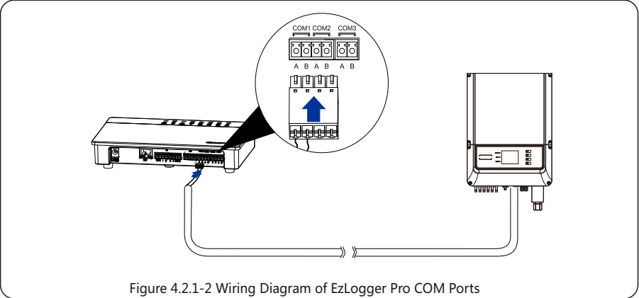
Figure 4.2.1-2 Wiring Diagram of EzLogger Pro COM Ports
